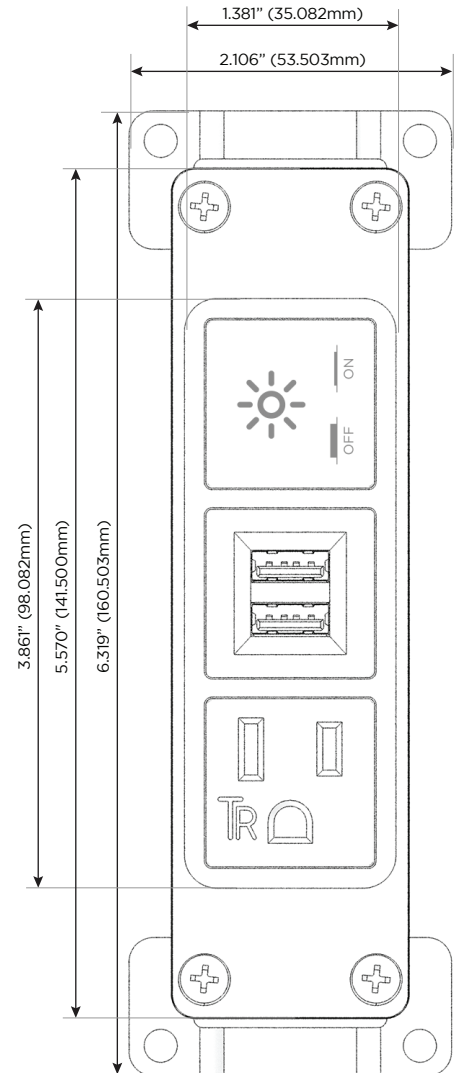
Shown with 1 Tamper Resistant AC, 1 Double USB Charging Port, and 1 Switched AC.
