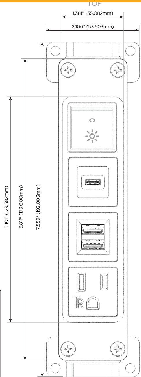
Shown with 1 Tamper Resistant AC, 1 Double USB Charging Port, 1 USB C Charging Port, and 1 Switched AC (Rocker Switch).
