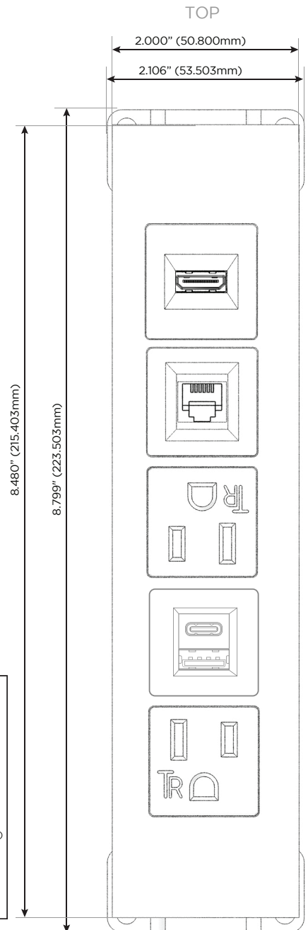
Shown with 2 Tamper Resistant ACs, 1 USB-A & 1 USB-C Charging Port, 1 RJ 12 Port, and 1 HDMI Port.
