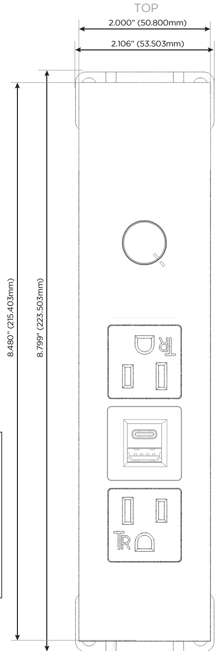
Shown with 2 Tamper Resistant ACs, 1 USB-A & 1 USB-C Charging Port, and 1 AC Dimmer.
